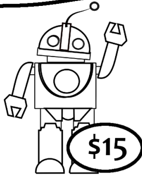
Robot
