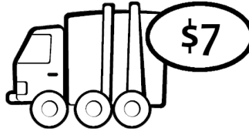
Toy Truck
